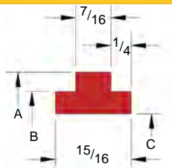
T-Shape Standard
